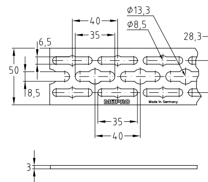
StaboFix® Rail
